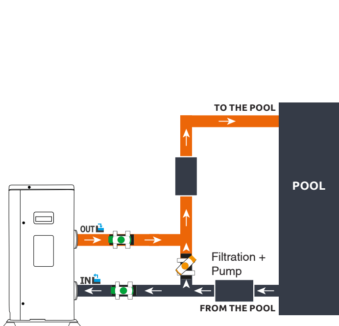
Simple assembly
